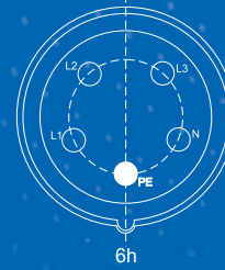
Position of the Earthing Contact
